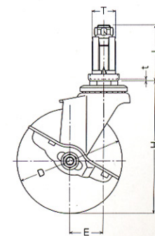
415EU-PR 100mm
